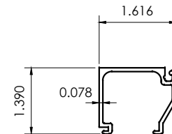
A3 GLASS STOP CG500-3
