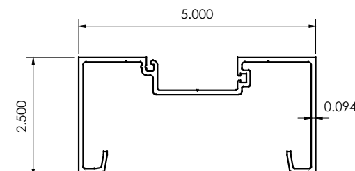
A4 LIGHT VERTICAL MULLION CG501-4
