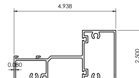
A4 LIGHT VERTICAL MULLION CG501-4
