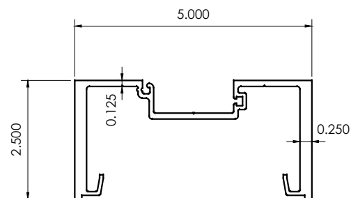
A7 HVY. VERTICAL MULLION CG501-7
