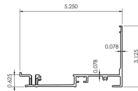
A10 STARTER SILL (HIGH) CG501-39
